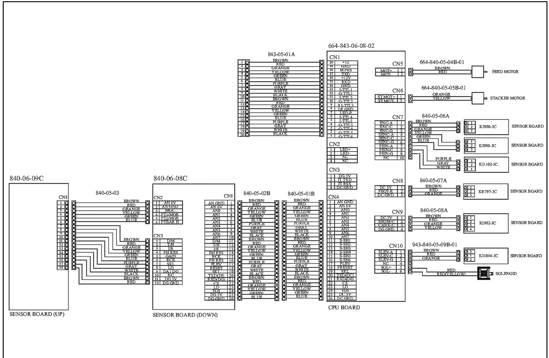
Figure 5-3 WBA-15-SS3B Bill Acceptor System Wiring Diagram
