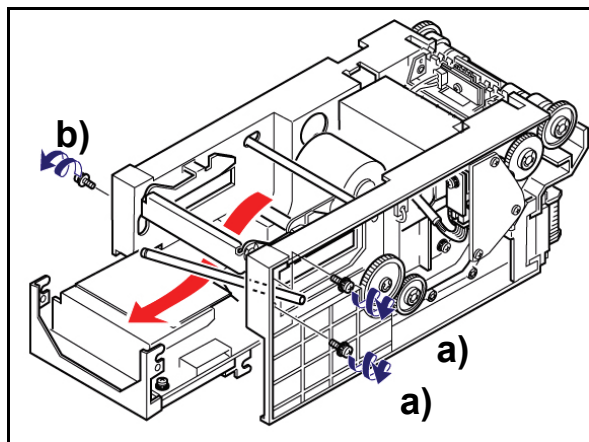
Figure 4-14 WBA Transport CPU Board Assembly Removal
