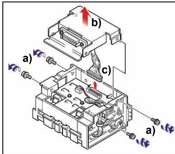
Figure 4-6 WBA Acceptor's Lower Sensor Board Cover Removal
