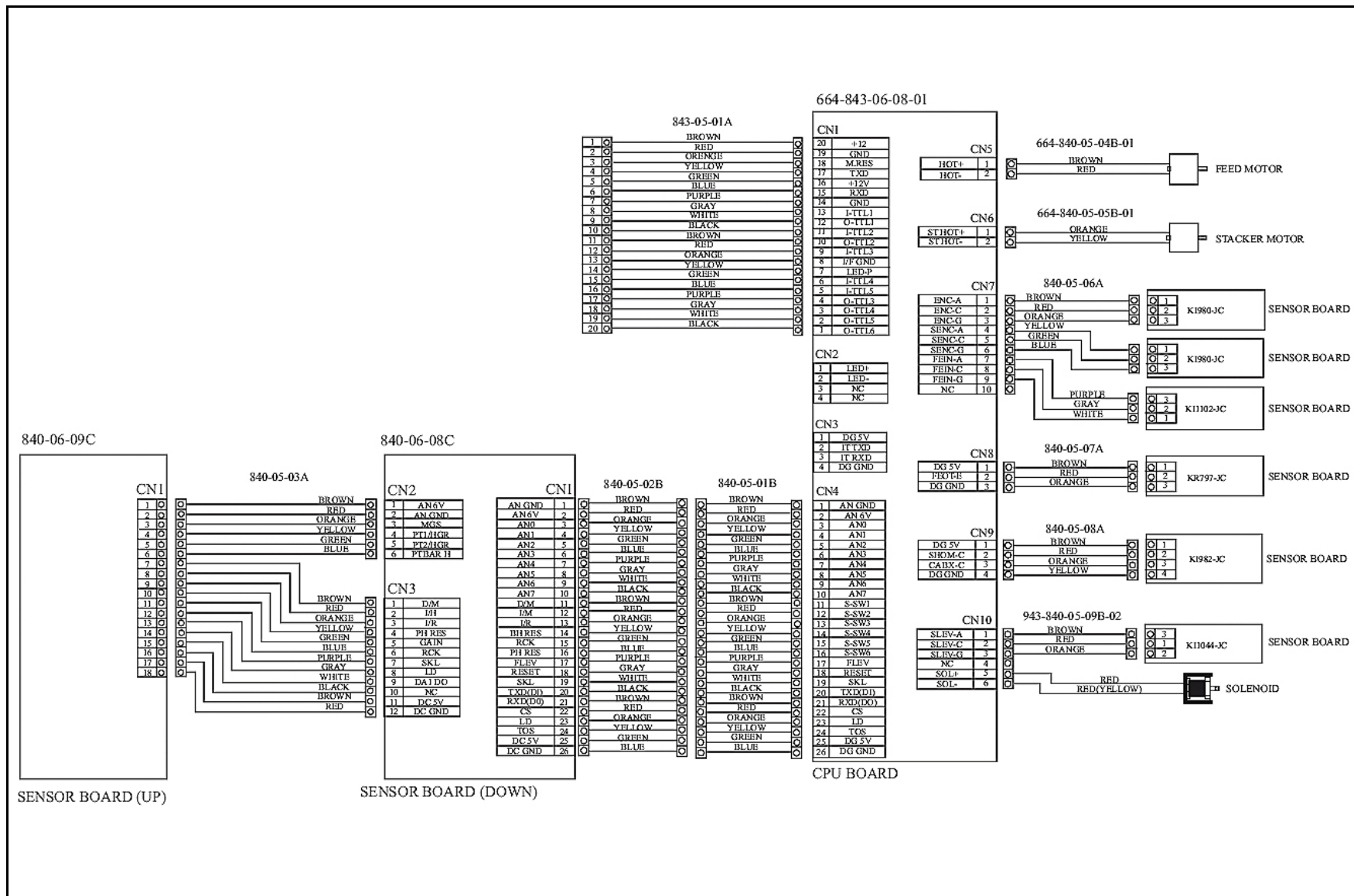
Figure 5-2 WBA-14-SS3B Bill Acceptor System Wiring Diagram
