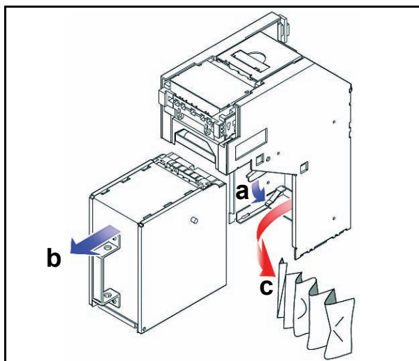
Figure 2-14 Clearing a Cash Box Inlet Bill Jam
