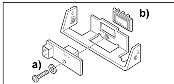
Figure 4-26 Transport Feed-Out Sensor Disassembly
