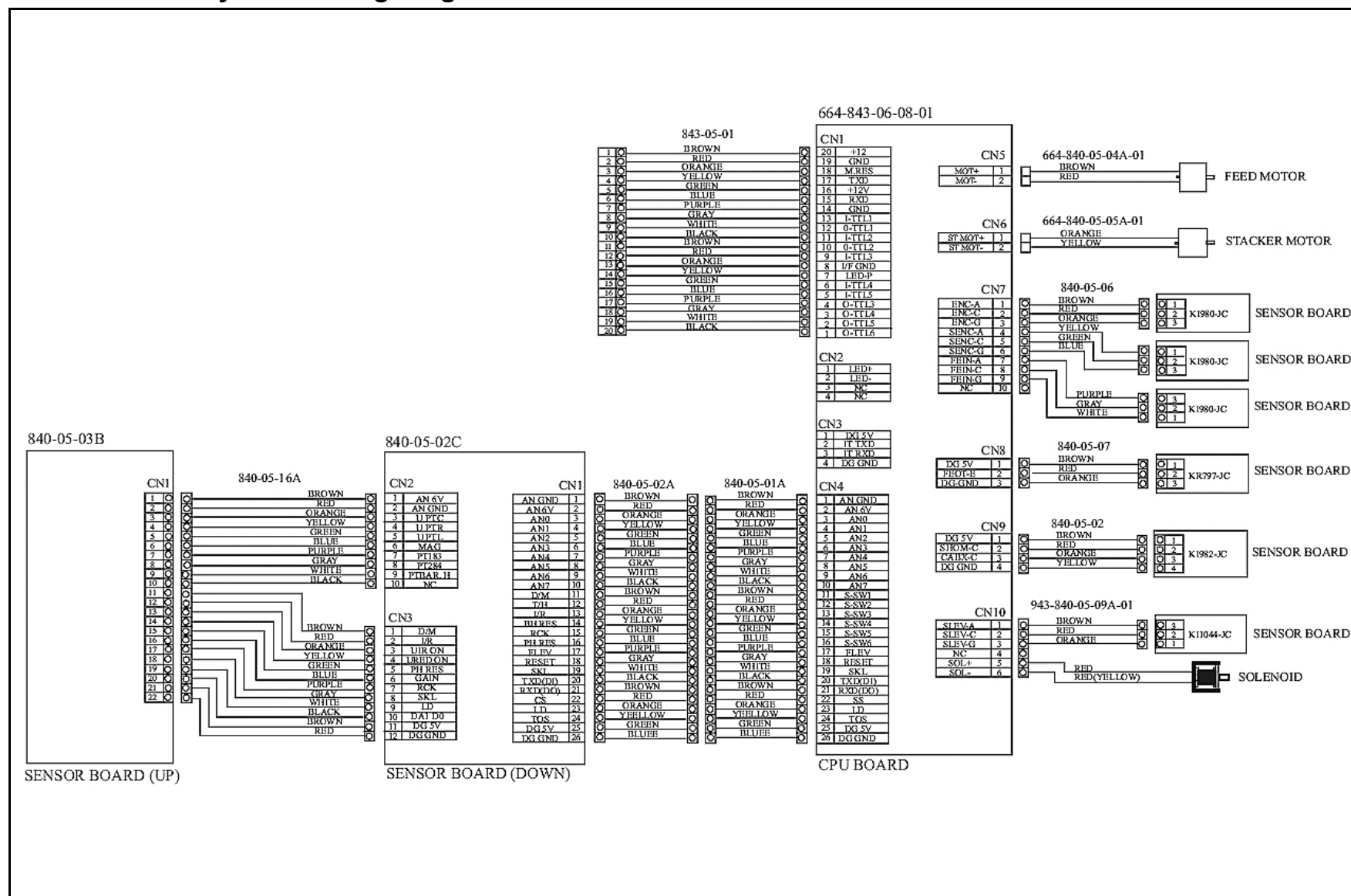
Figure 5-4 WBA-24-SS3B Bill Acceptor System Wiring Diagram
