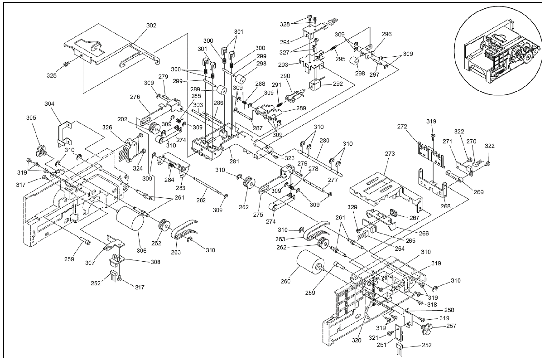
Figure 7-6 WBA Transport Unit Exploded View (Part 3)
