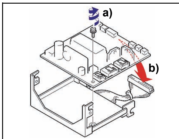
Figure 4-15 Transport CPU Board Removal
