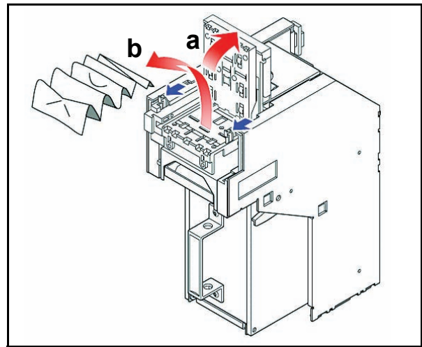
Figure 2-12 Clearing an Entrance Bill Jam
