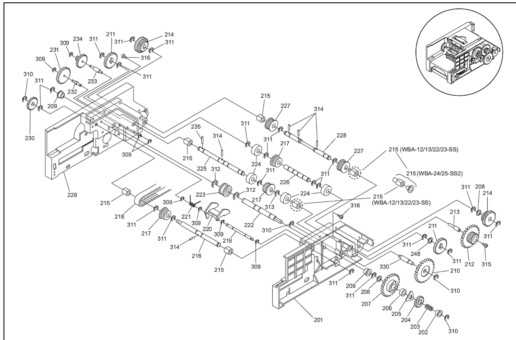
Figure 7-4 WBA Transport Unit Exploded View (Part 1)
