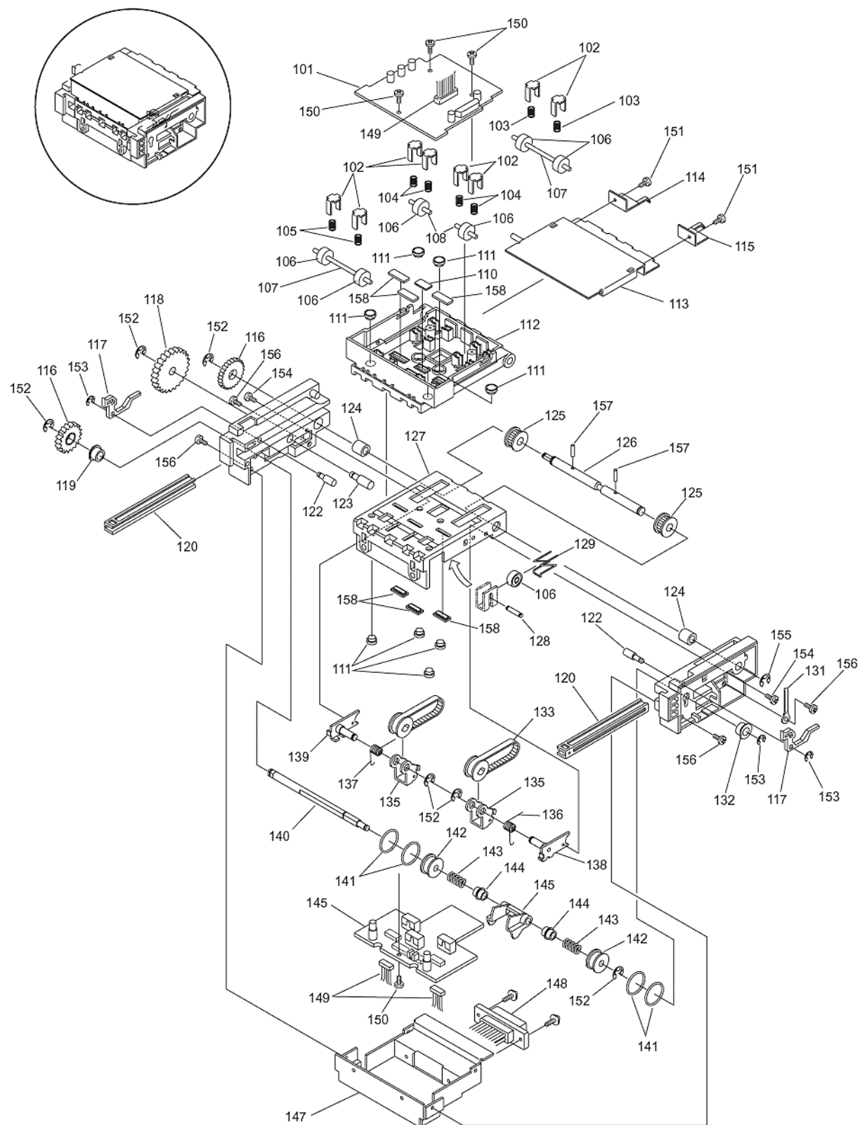
Figure 7-3 WBA 22/23/24/25 Acceptor Head Exploded View
