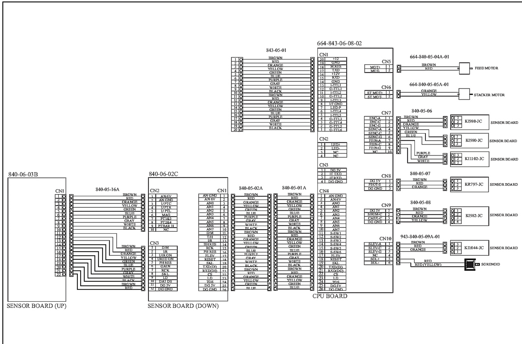
Figure 5-1 WBA-25-SS3B Bill Acceptor System Wiring Diagram
