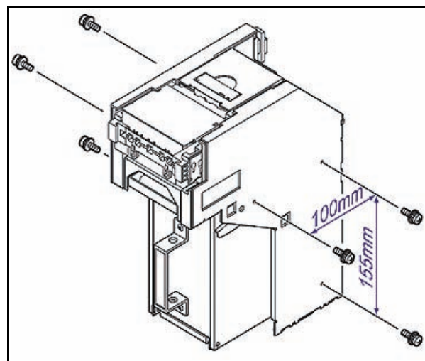
Figure 2-2 Side Mounting Screw Hole Locations
