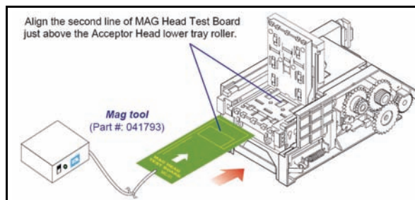
Figure 6-18 Aligning the MAG Head Calibration Test Board
