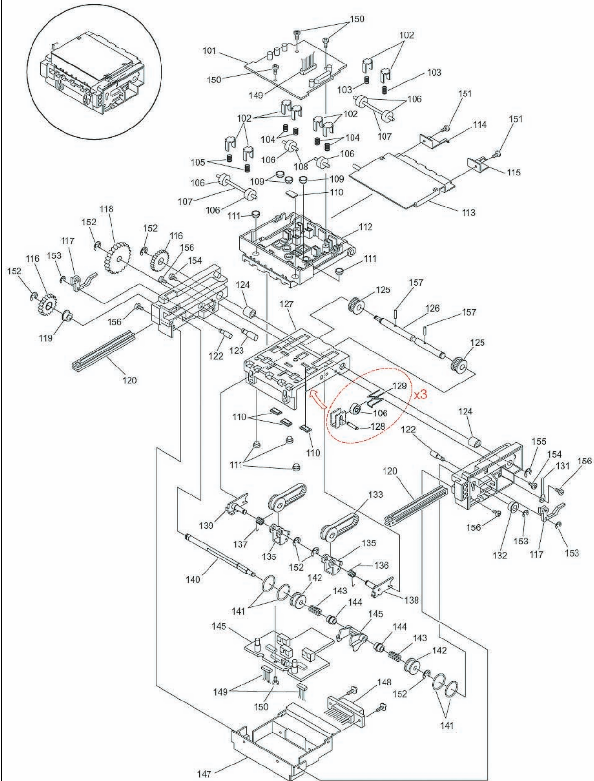
Figure 7-2 WBA 12/13 Acceptor Head Exploded View
